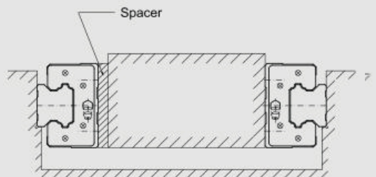
Back-to-back configuration
