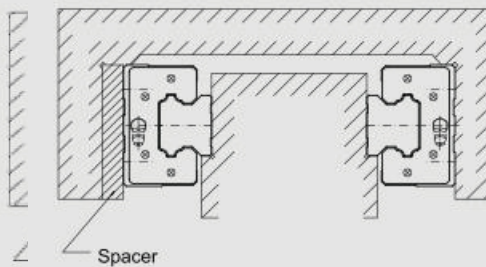
Vertical Configuration.
