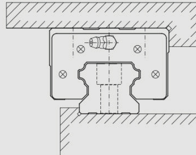
Upside down Configuration.
