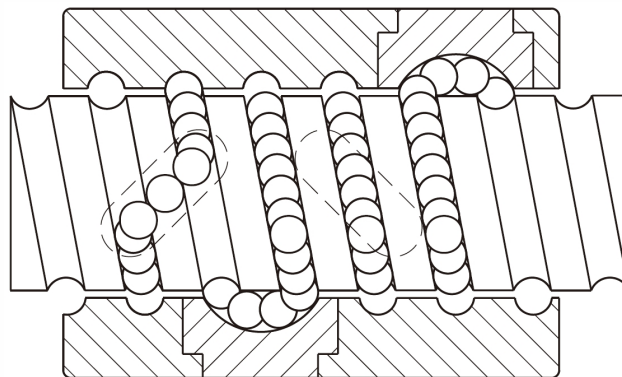
Fig 1.6.1 U, I - Type Nut
