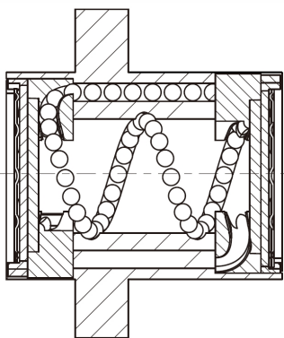
Fig 1.6.4 Y, YA, A, J - Type nut
