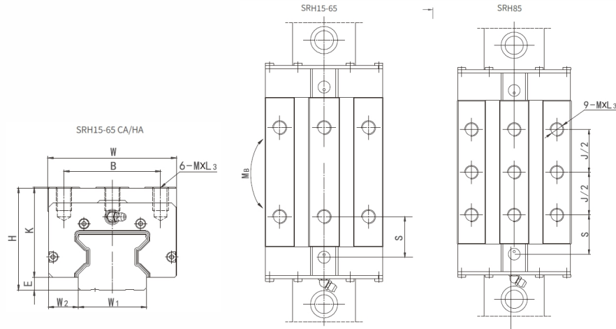
SR Series Size CA Rectangular Slide Block HA Extended Rectangular Slide Block
